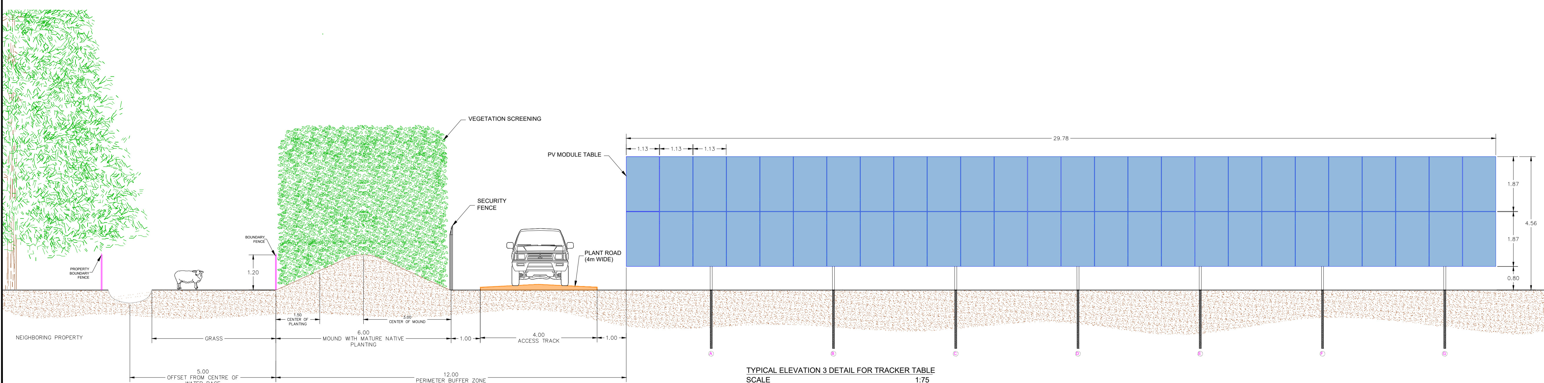
TYPICAL ELEVATION 2 DETAIL FOR TRACKER TABLE SCALE 1:75
