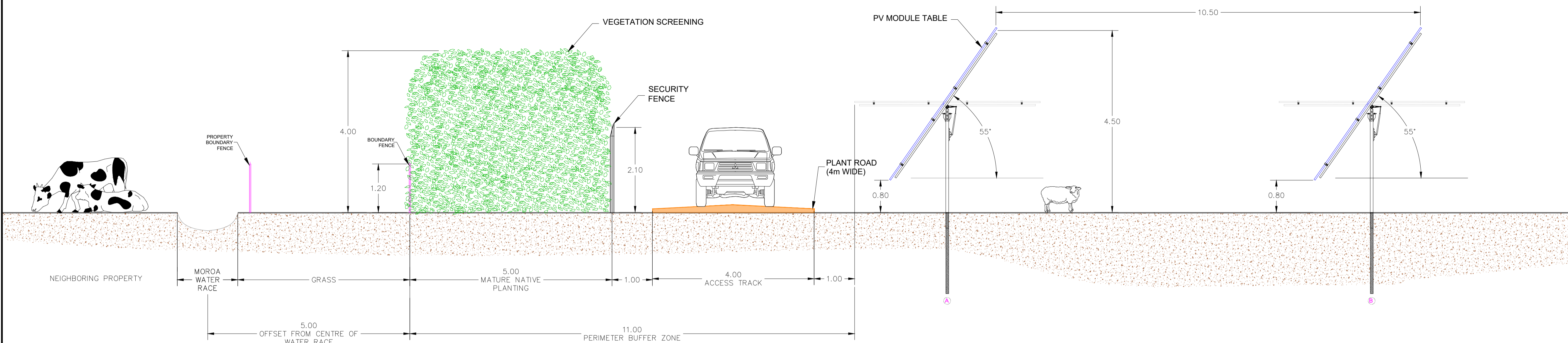
TYPICAL ELEVATION 1 DETAIL FOR TRACKER TABLE SCALE 1:55
